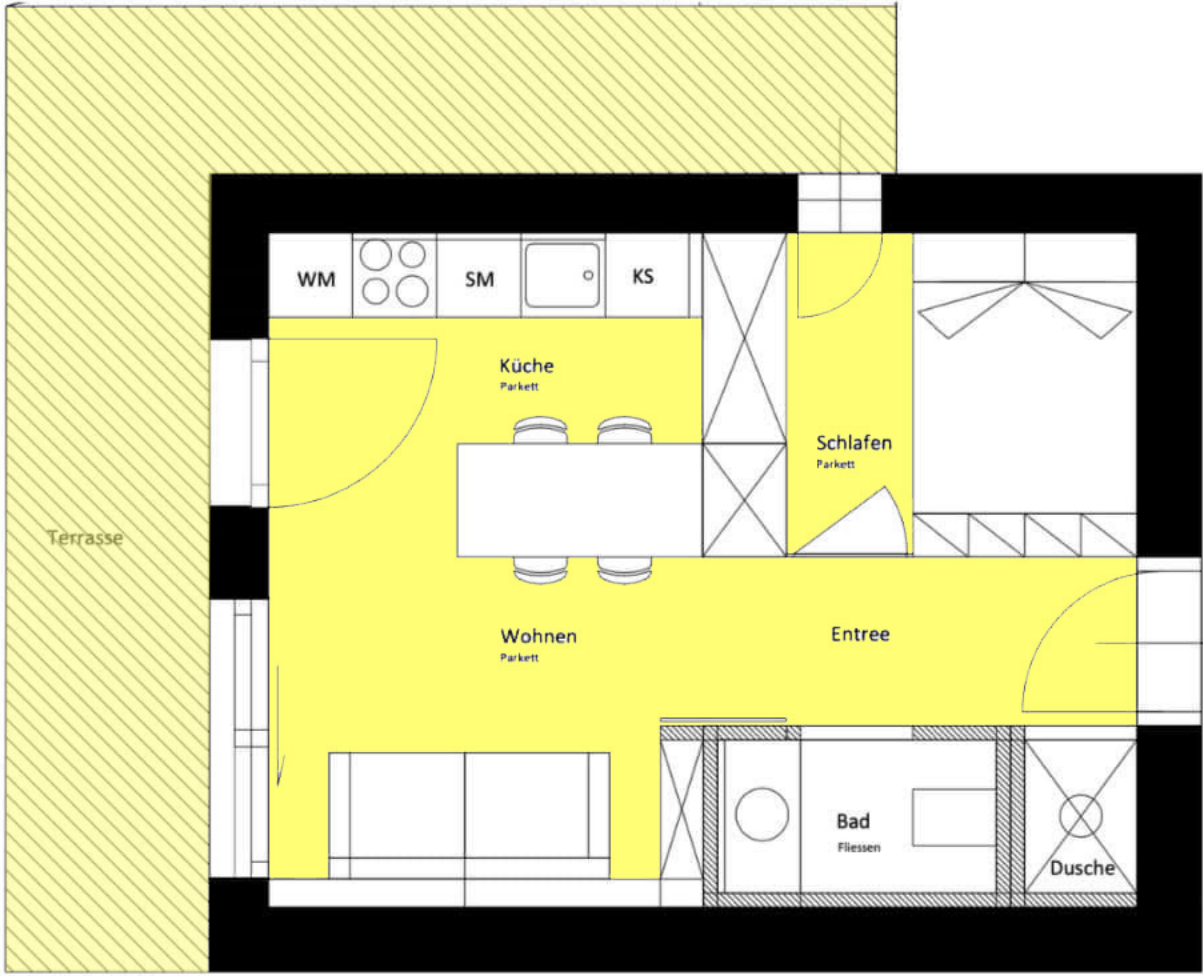
ERDGESCHOSS - PIANO TERRA
